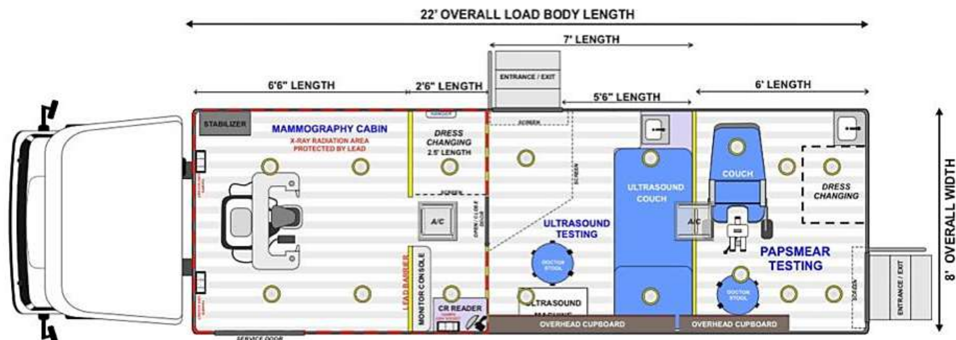
MOBILE MAMMOGRAPHY ON WHEELS ASHOK LEYLAND 1415HB / 4900MM WB
